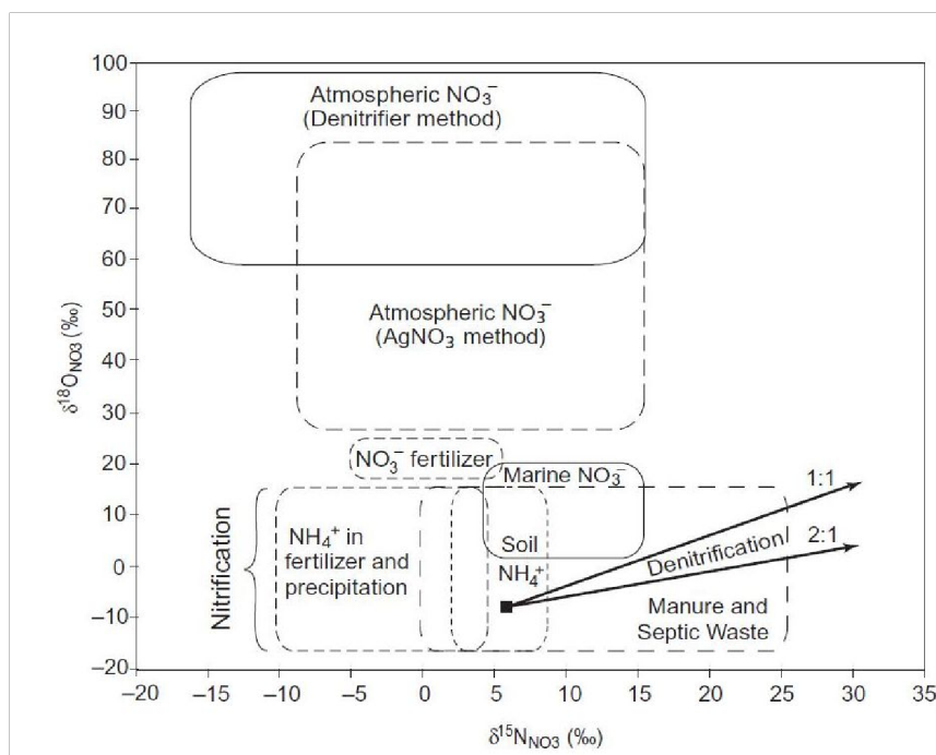
Figure 22. Typical values of the Stable Isotopes of oxygen ( \delta^{18}\text{O} ) and nitrogen ( \delta^{15}\text{N} ) of nitrate derived from various sources (diagram from
